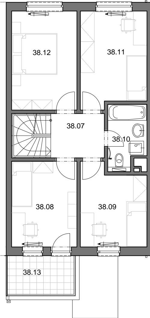
PŮDORYS 2.NP / LAYOUT 2nd AGF
